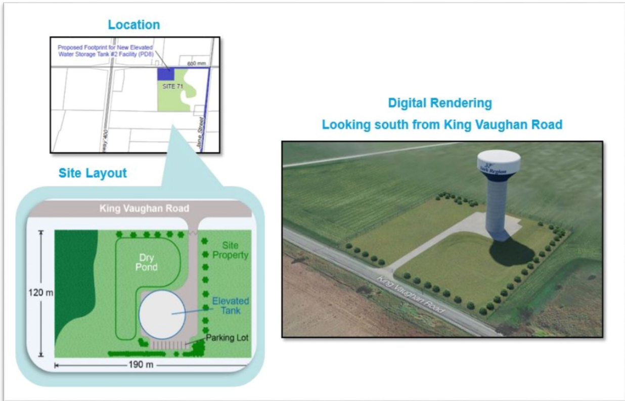
Figure E. 12 Proposed Location, Site Layout and Rendering of the Pressure District 8 Second Elevated Tank at Site 71
