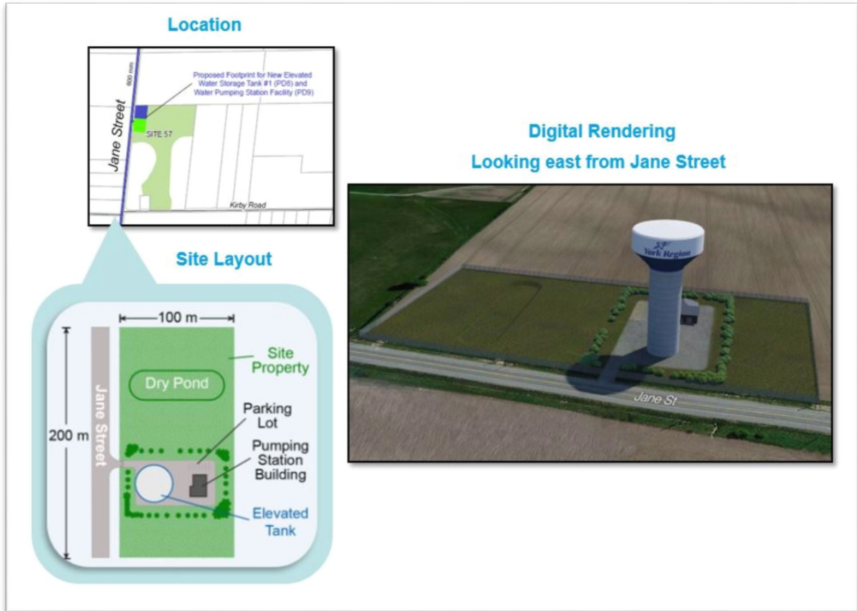
Figure E. 11 Proposed Footprint Location, Site Layout and Rendering of the Combined Pressure District 8 Elevated Tank and Pressure District 9 Pumping Station at Site 57
