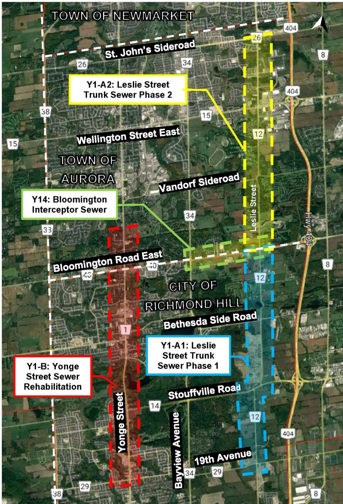
Figure 6.1 Overview of Leslie Street Trunk Sewer and Yonge Street Sewer Rehabilitation Projects
