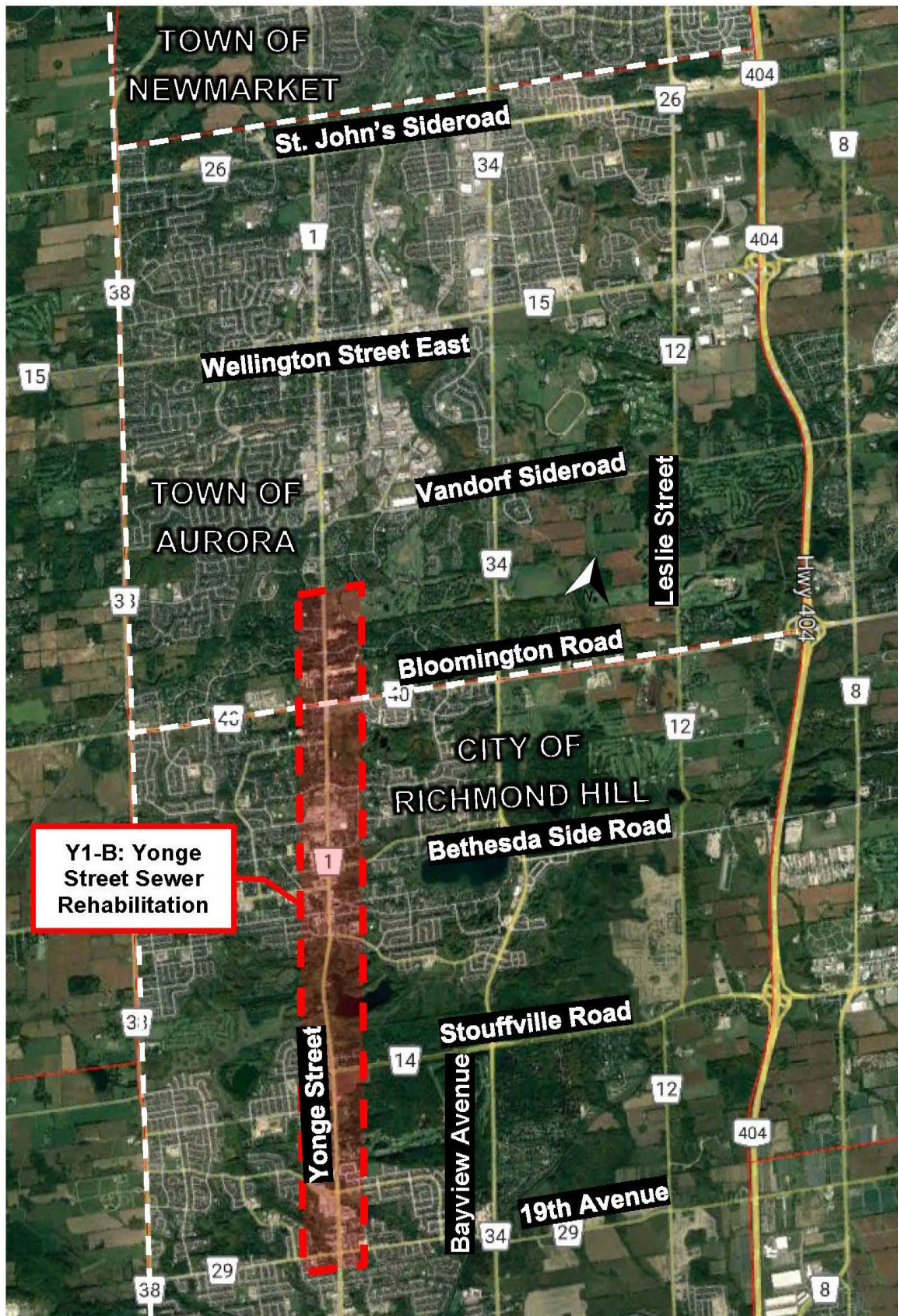
Figure 6.17 Overview of Y1-B Yonge Street Sewer Rehabilitation Project
