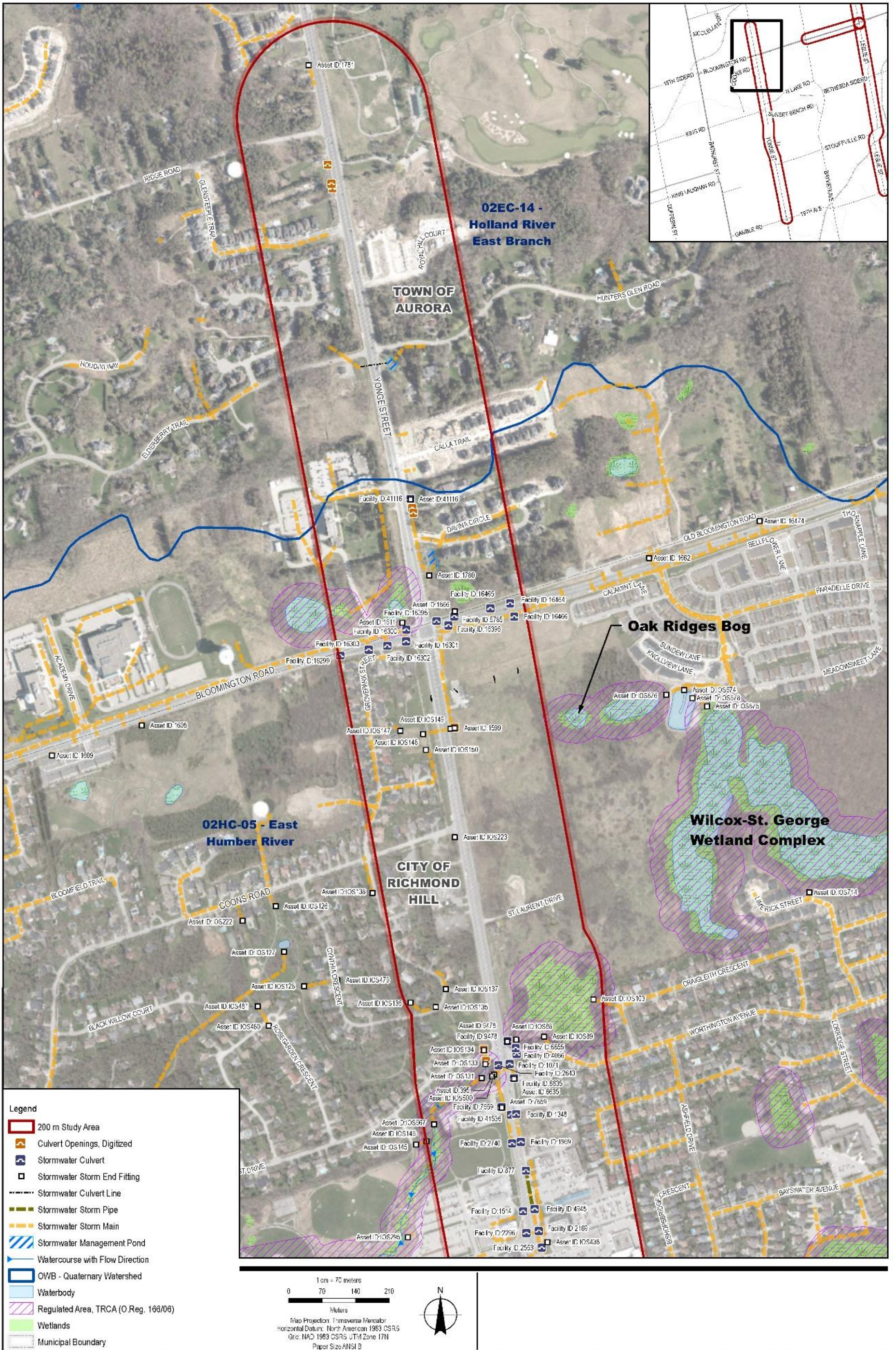
Figure 6.20 Y1-B Study Area Surface Water Map for Existing Conditions, North Section
