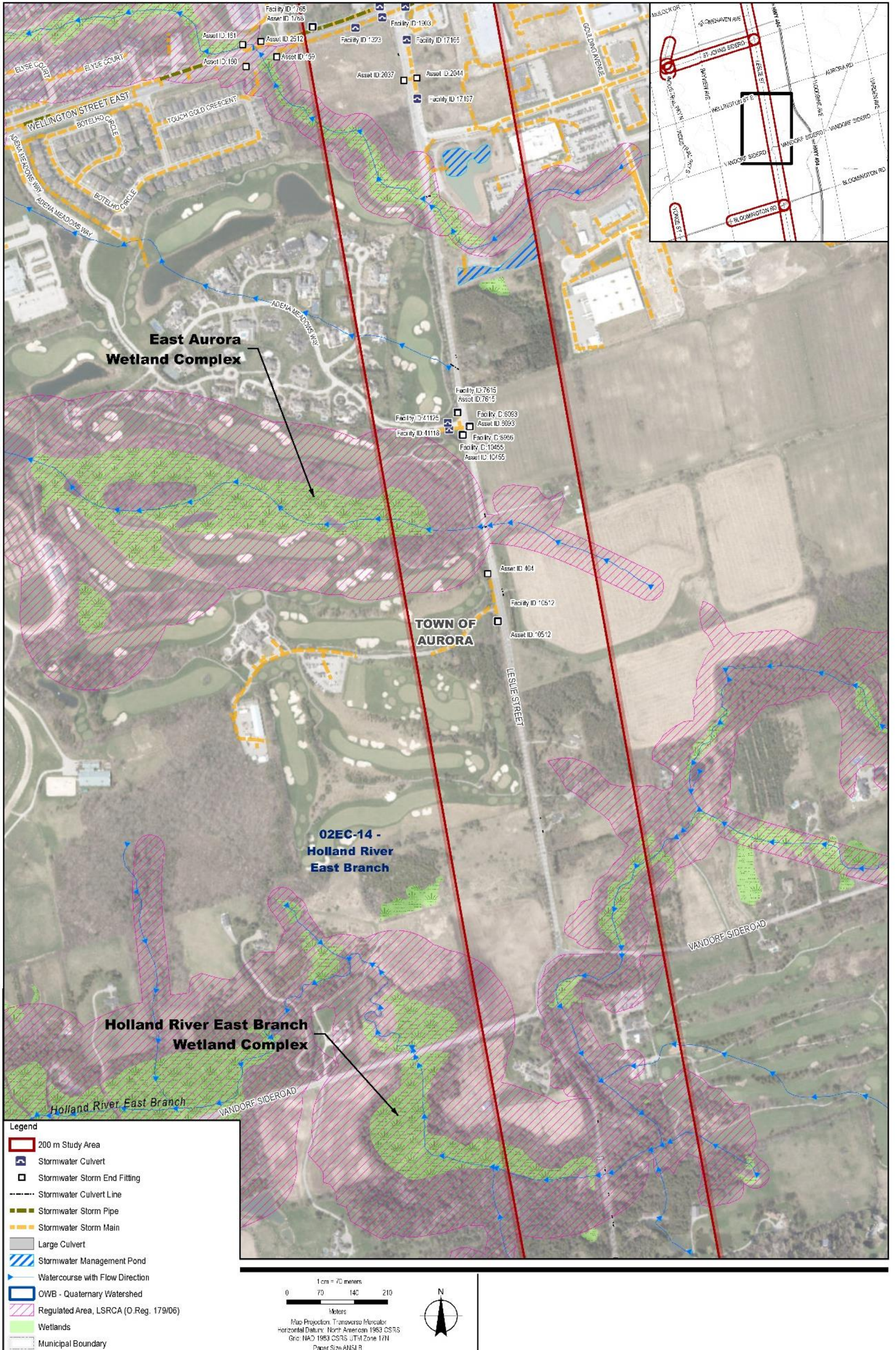
Figure 6.13 Y1-A2 Study Area Surface-Water Map of Existing Conditions, Middle Section
