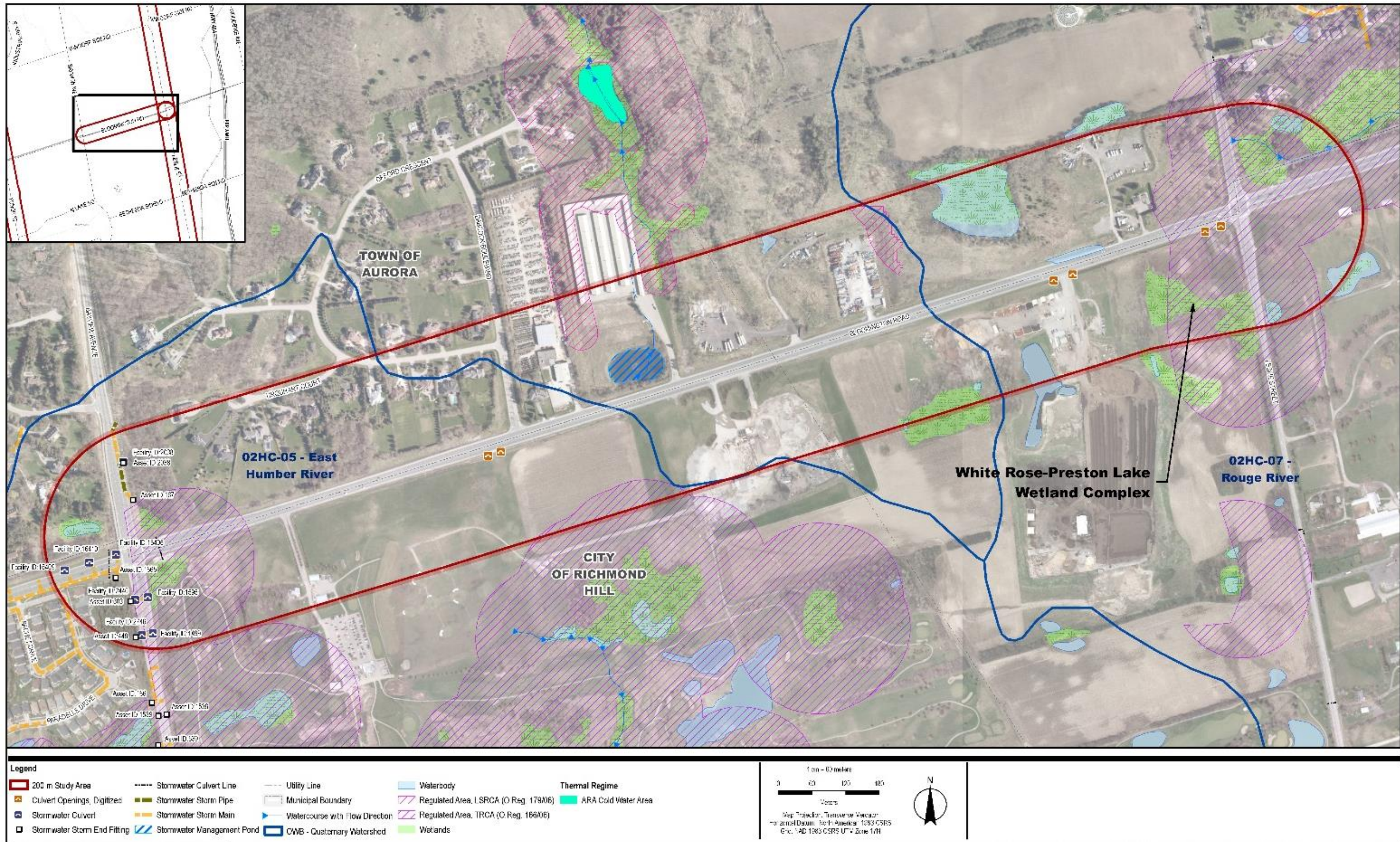
Figure 6.15 Y14 Study Area Surface Water Map of Existing Conditions
